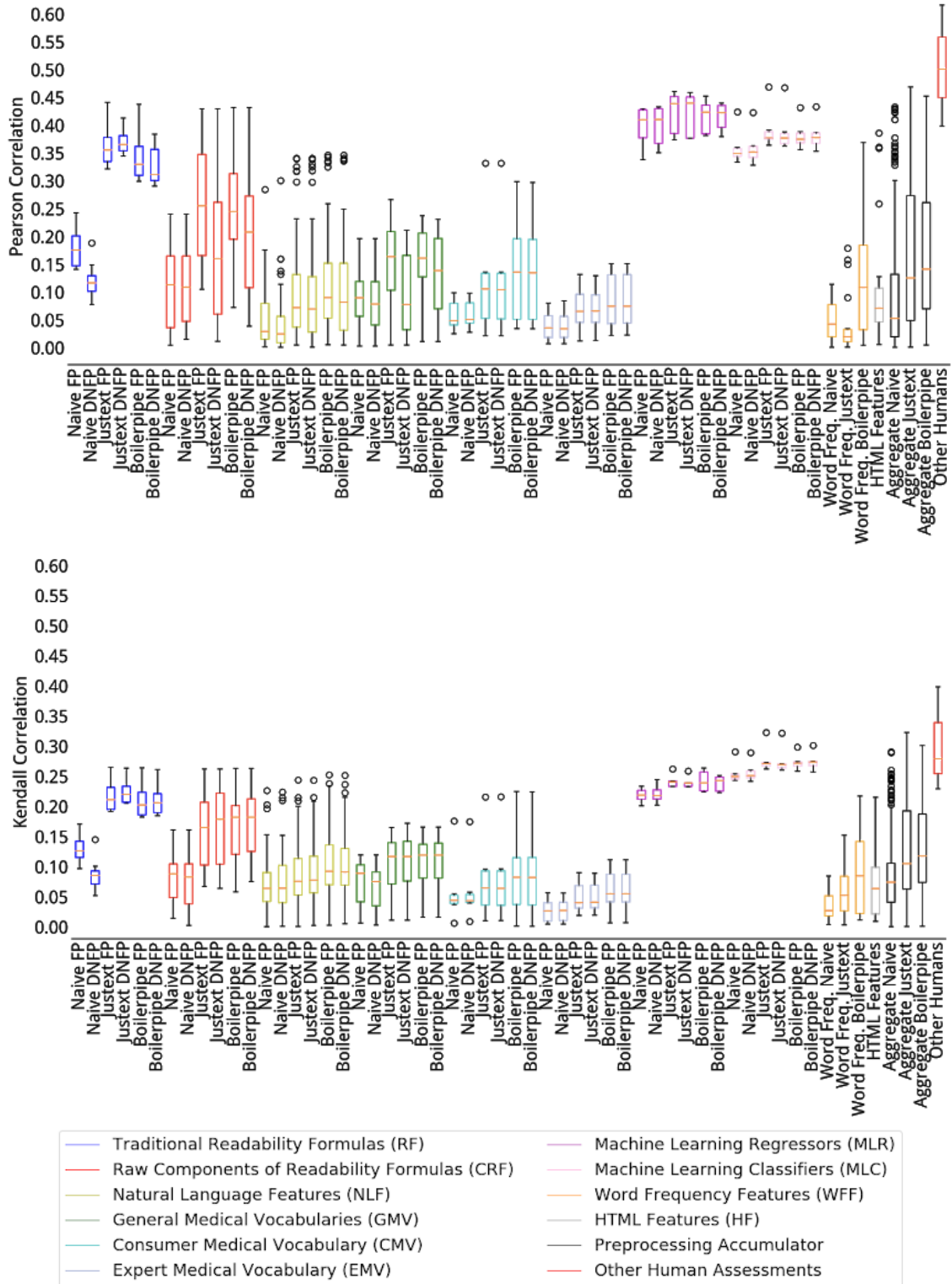
Figure 2. Correlations between understandability estimators and human assessments for CLEF 2016.
